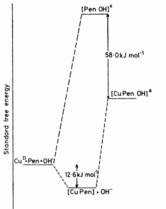
FIGURE 4 Plot of the standard free-energy change for the copper(II) catalysed hydrolysis of benzylpenicillin compared with the hydroxide-ion catalysed reaction at a standard state of 1M
