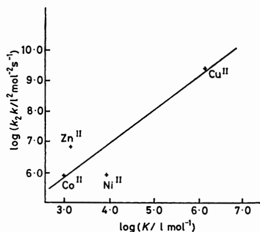
FIGURE 5 Plot of the logarithm of the third-order rate constants at 30° for the metal-ion and hydroxide-ion catalysed hydrolysis of benzylpenicillin against the logarithm of the association constants of thioproline and metal ion at 25°
