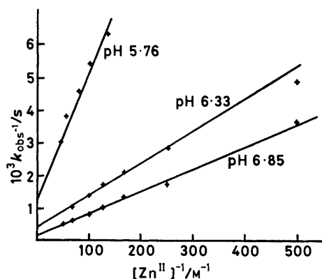
FIGURE 2 Plot of the reciprocal of the apparent first-order rate constant for the hydrolysis of benzylpenicillin in cacodylate or acetate buffers at 30.0°C and at the pH values indicated as a function of the reciprocal of the zinc(II) concentration
