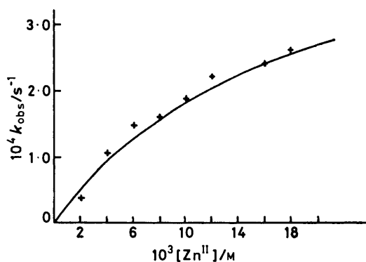
FIGURE 1 Plot of the apparent first-order rate constant for the hydrolysis of benzylpenicillin at pH 5.81 and 30.0°C ( I 0.50M) as a function of total zinc(II) ion concentration. The solid line is calculated from the constants given in the text
